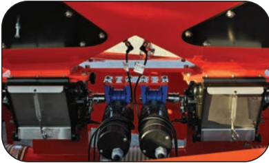
Single shot seed and fertiliser distribution system
